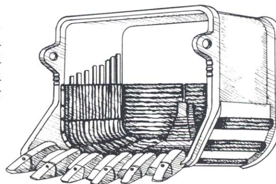
SHOVEL BUCKET LINER
